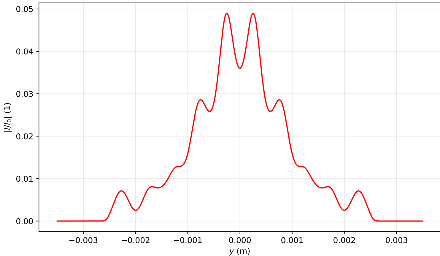
Intensity profile I(x = 0, y, z = 3.821)/I_0 , P_{in}=2.0P_{cr} , artificial time
